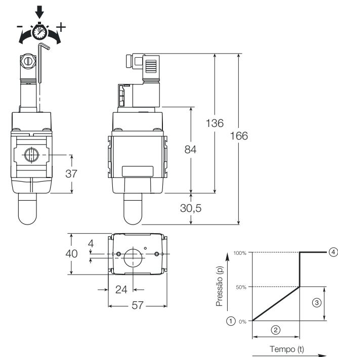
P31TA - 1/4"
