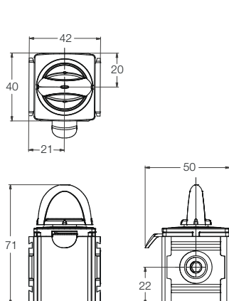
P31VB - G 1/4"
