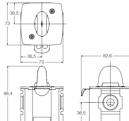
P33VB - G 3/4"
