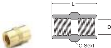
207P - Luva NPTF / SAE 130138
