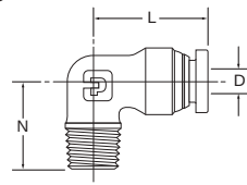
W169PLPNS - Cotovelo macho Tubo / macho NPTF
