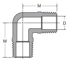
1204P - Cotovelo macho NPTF
